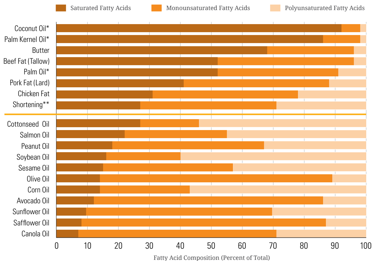
Figure 1-2. Fatty Acid Profiles of Common Fats & Oils
